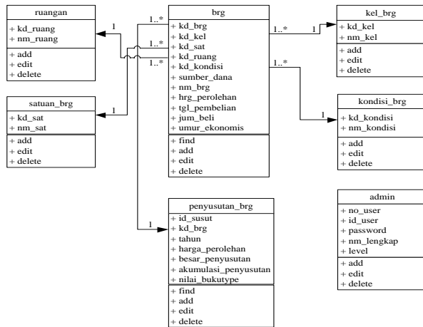
Gambar 3. Class Diagram
